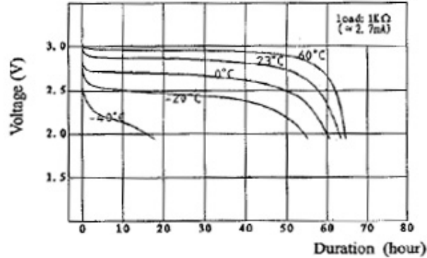
Discharge curve at various temperatures
