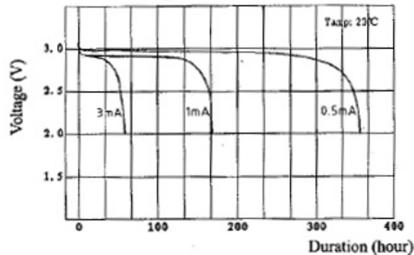
Discharge curve at various currents
