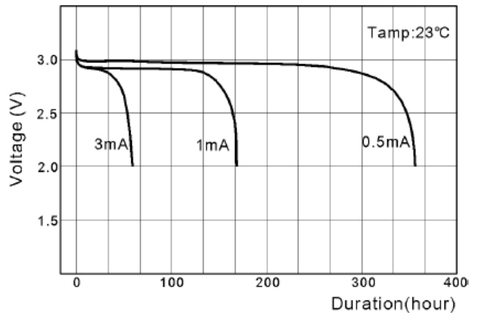
Discharge curve at various currents
