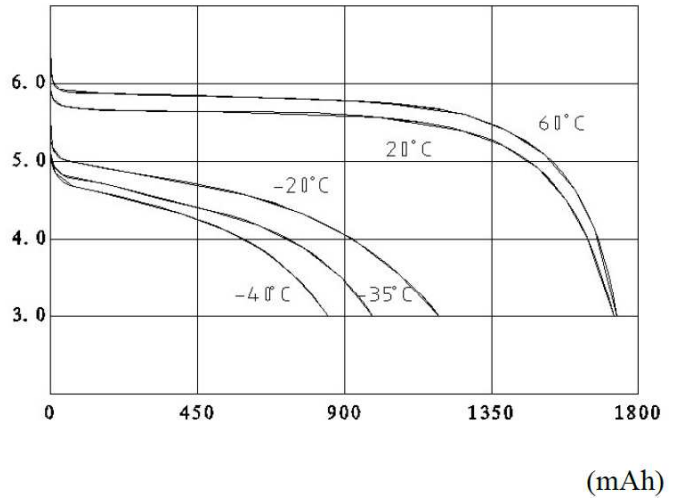
Pulse discharge characteristics
